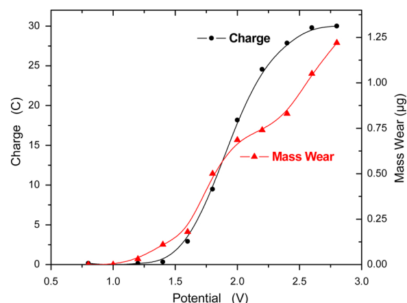
Fig. 3. Electrochemical system bias curve and electrode mass wear.
