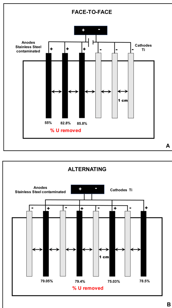
Fig. 7. Efficiency of removal of U by EC as a function of the electrochemical cell configurations, in face-to-face (A) and alternate (B).
