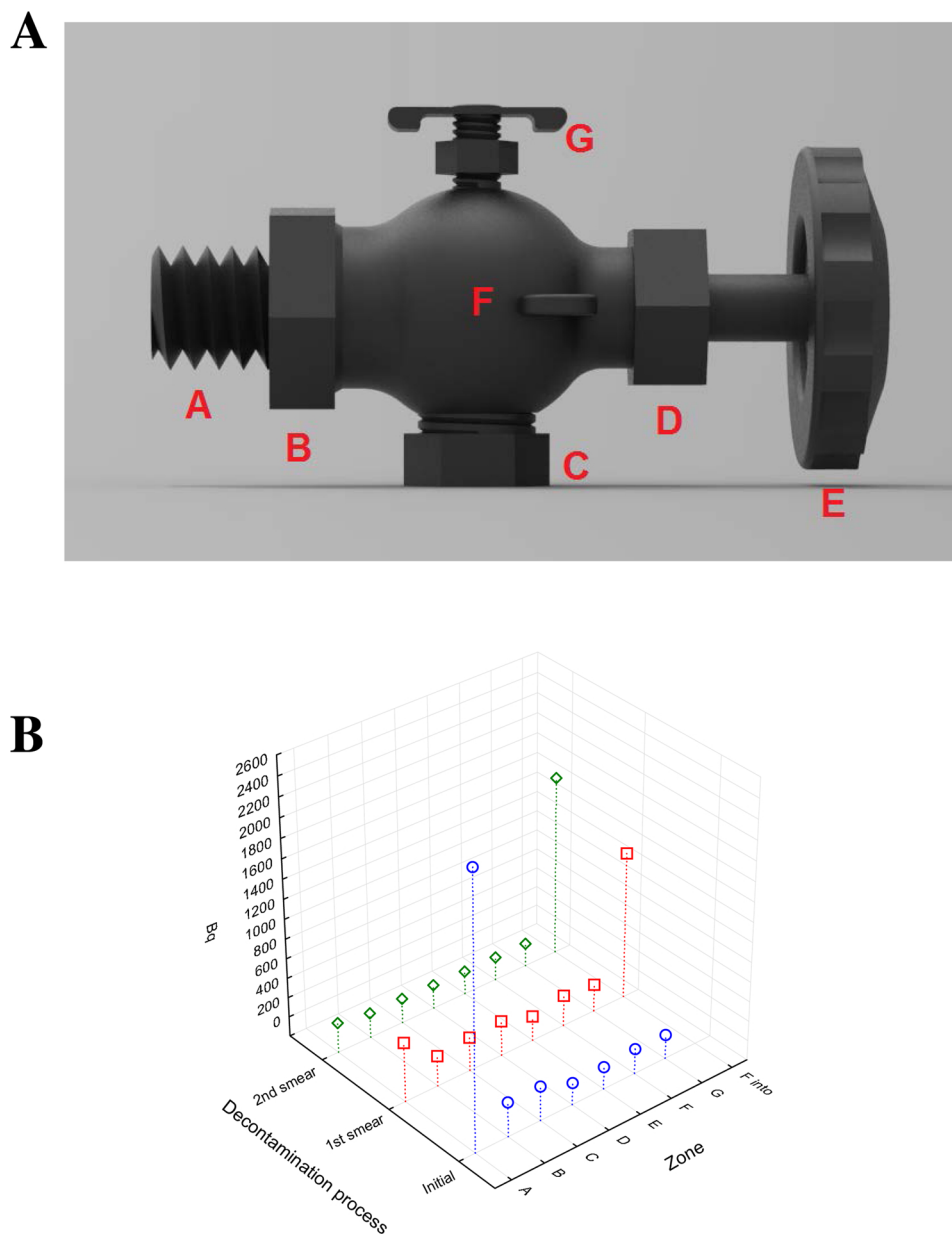
Fig. 9. Division into zones of Piece #1 (A) and Contamination levels of Piece #1 in Bq during the decontamination process (B).
