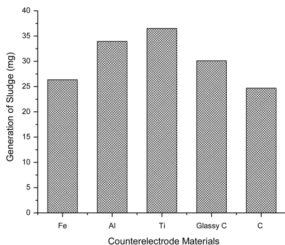
Fig. 5. Generation of sludge (LW) according to the type of counter electrode applying the EC process for 1 h.
