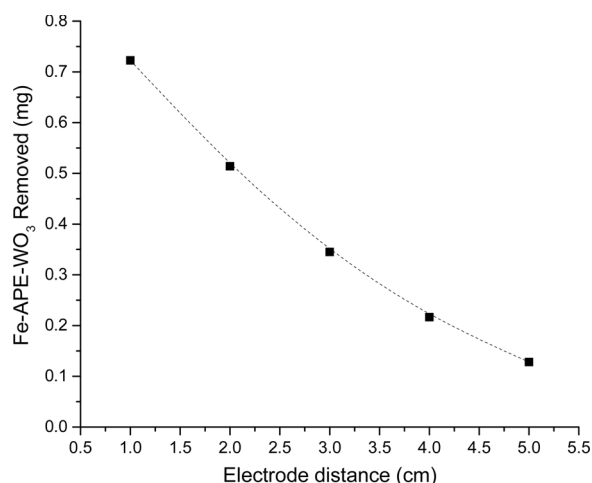
Fig. 4. Removal of \text{WO}_3 as a function of the anode distance (W-EPA |A) / cathode (Fe).
