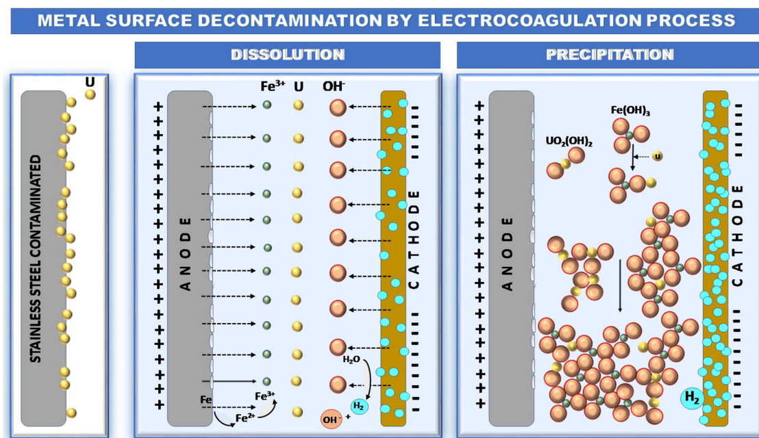
Fig. 8. Mechanisms of U decontamination by electrocoagulation process.
