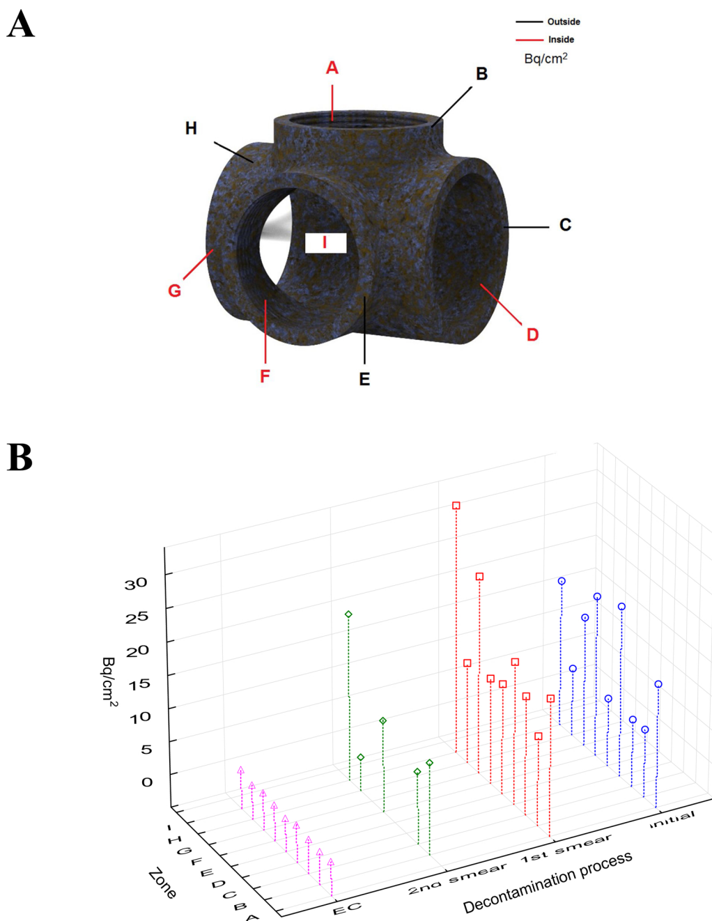
Fig. 11. Division into zones of Piece #2 (A) and Contamination levels of Piece #2 in Bq/cm 2 during the decontamination process (B).
